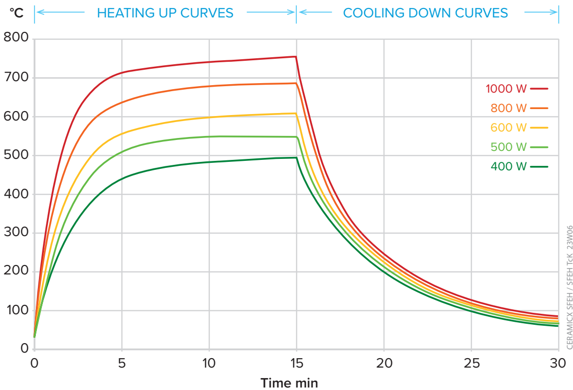
SFEH TcK Heat up and cool down curves showing average surface temperature measured with a thermal imaging camera set to an emissivity of 0.95 (element mounted in a polished aluminium clad steel reflector)
